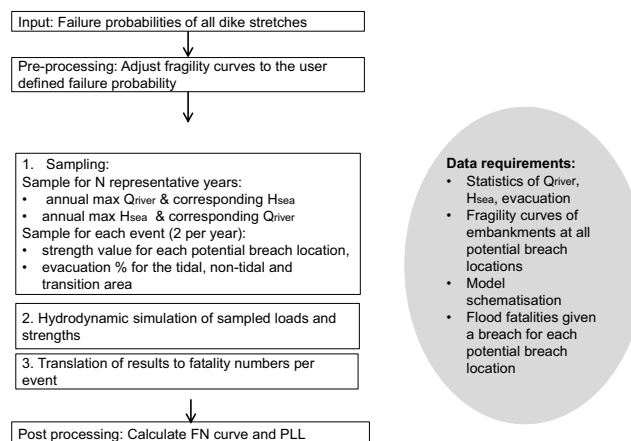
Figure 3. Schematic overview of the probabilistic risk assessment method for river deltas (adapted from [3])
