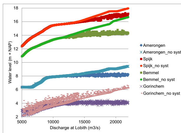
Figure 8. Relation between maximum discharges at Lobith and maximum water levels at various locations assessed with and without taking hydrodynamic interdependencies into account (without = no syst)
