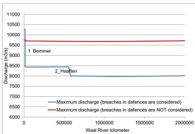
Figure 6. Waal maximum discharges in the example event
