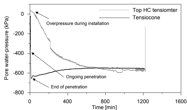
Figure 14. Penetration test in the laboratory
