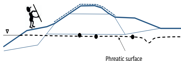
Figure 26. Inspection of the embankment cross-section using GEM2. The portion of the crest dashed indicates the segment where water depth was predicted based on GEM2 data.
