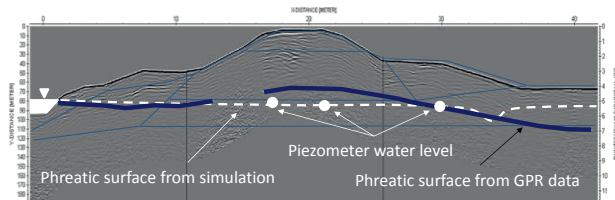
Figure 20. GPR data interpretation for the Adige river embankment, November 2014 (K452).
