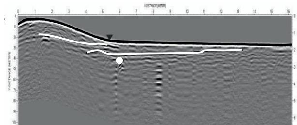
Figure 21. GPR data interpretation for the Leendert de Boerspolder embankment (K234)
