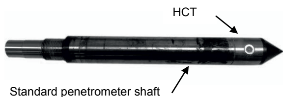
Figure 12. Prototype penetrometer shaft
