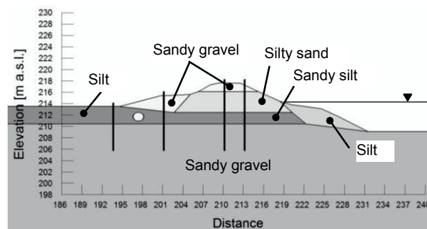
Figure 18. Cross section of the Adige river flood embankment
