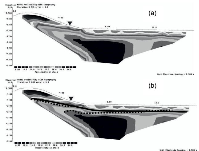
Figure 25. ERT data from the De Leendert de Boerspolder embankment. (a) Raw ERT data. (b) Phreatic surface drawn by integrating ERT and GPR data.
