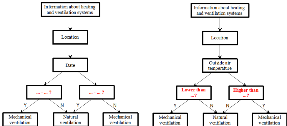
Fig. 4. Control algorithm for seasonal strategy (left) and outside air temperature strategy (right).
