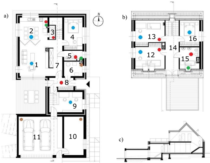
Fig. 6. Research object – detached house located near Wrocław: a) ground floor, b) attic, c) cross-section [21].
