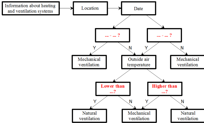
Fig. 5. Control algorithm for seasonal and outside air temperature strategy.
