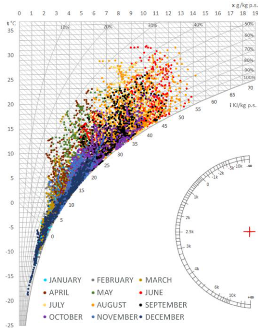
Fig. 3. The parameters of outside air – Wrocław.
