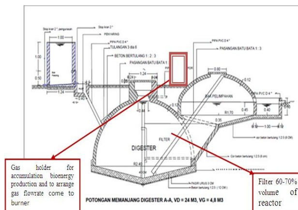
Fig. 1. Reactor Design for the process of Vinasse Digestion
