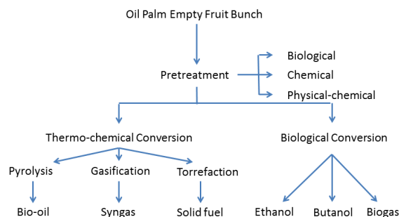
Fig.2. Biofuel production from OPEFB [23].
