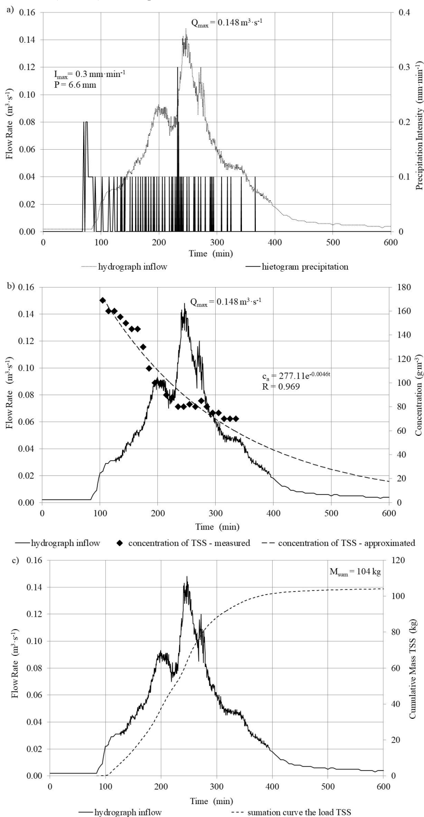
Fig. 2. Characteristics of selected peak rainfall runoff event of 05 May 2010 for IX Wieków Kielc SWTP catchment with respect to stormwater flow rate, precipitation intensity, and also concentration and mass of TSS.
