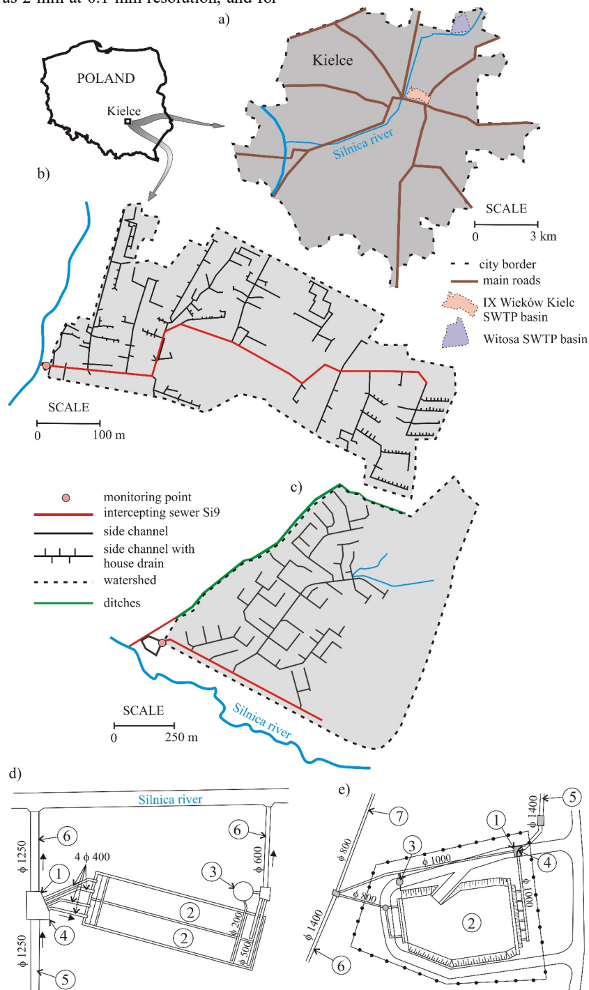
Fig. 1. Study area: a) location in the city of Kielce, b) IX Wieków Kielc SWTP catchment, c) Witosa SWTP catchment, d) scheme of the IX Wieków Kielc SWTP, e) scheme of the Witosa SWTP; 1 - separation chamber; 2 - horizontal settling tank; 3 - coalescence separator; 4 - regulated stormwater overflow; 5 - inflow of stormwater, 6- outflow to the river Silnica, 7- inflow from the ditch.
