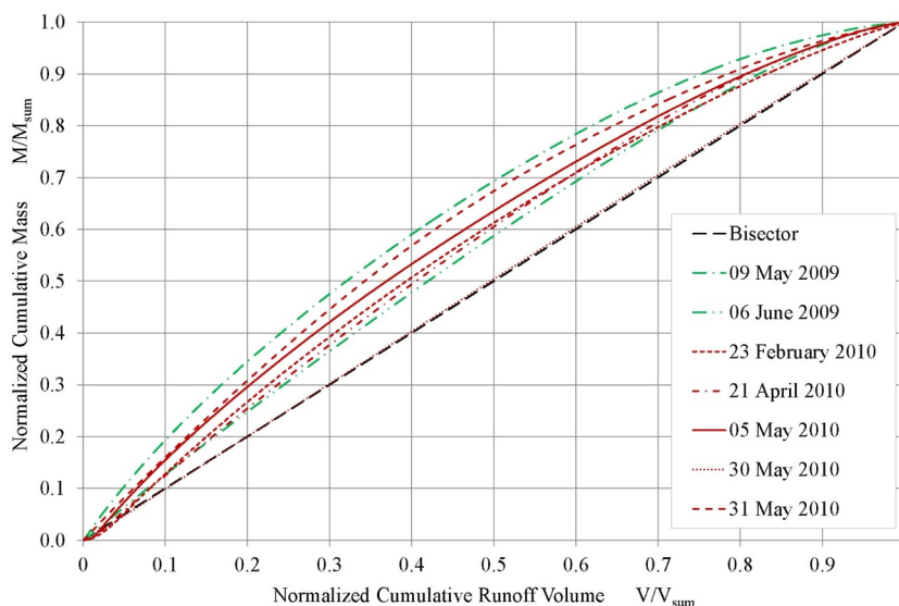
Fig. 4. Dimensionless curves of cumulative TSS mass vs. cumulative discharged volume for IX Wieków Kielc SWTP catchment.
