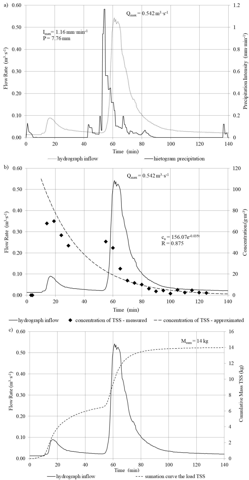
Fig. 3. Characteristics of selected peak rainfall runoff event of 20 May 2015 for Witosa SWTP catchment with respect to stormwater flow rate, precipitation intensity, and also concentration and mass of TSS.
