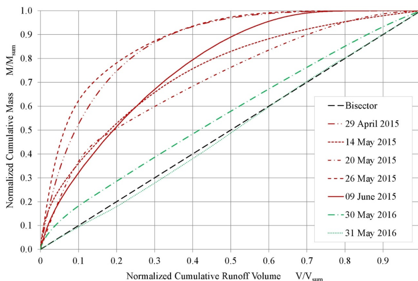
Fig. 5. Dimensionless curves of cumulative TSS mass vs. cumulative discharged volume for Witosa SWTP catchment.
