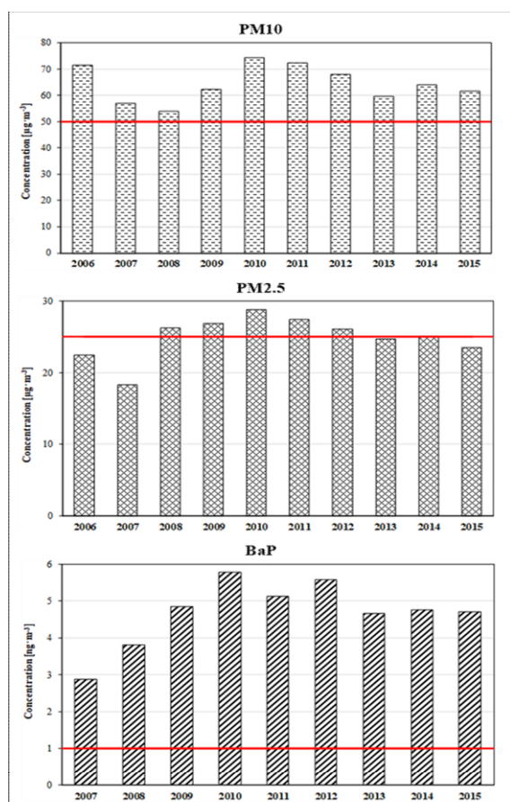
Fig. 1. Concentration of PM10, PM2.5, BaP in Poland [5].
