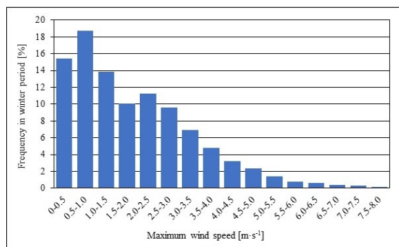
Fig.4. Distribution the frequency of occurrence the maximum wind speeds in winter period.
