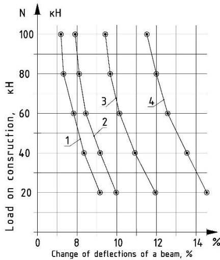
Fig. 2. The change in the calculated deflections of wooden beams of the composite section with increasing wood moisture: 1 - 6 to 12%, 2 - 12 to 18%, 3 - 18 to 24%, 4 - from 24 to 30%.
