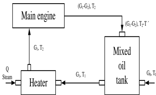
Fig. 1. The working procedures of the fuel oil viscosity and temperature control system.
