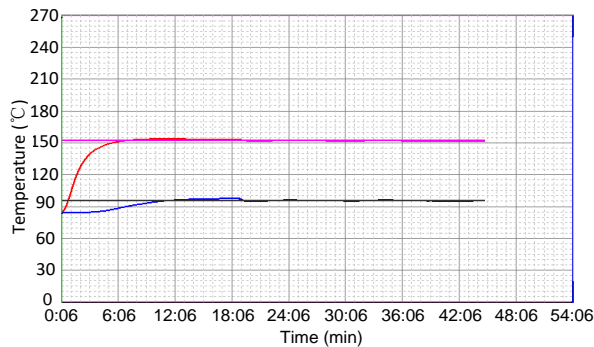
Fig. 3. The fuel oil temperature control experiment of SMVS.
