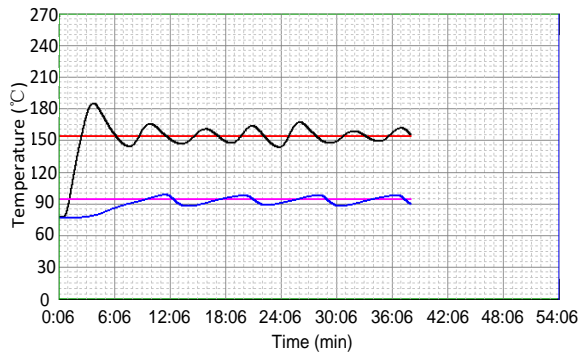
Fig. 2. The fuel oil temperature control experiment of PID.
