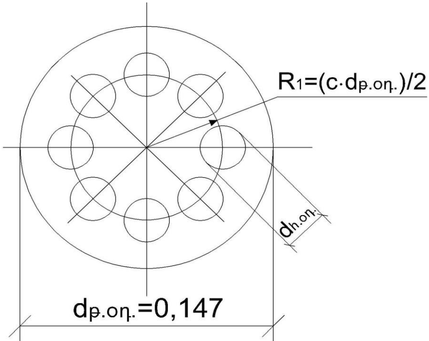
Fig.1. Eight-pipe recuperator of “pipe in pipe” type
