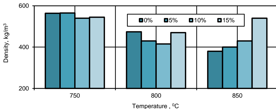
Fig. 3. The effect of pyrite additive on density of burnt granules.
