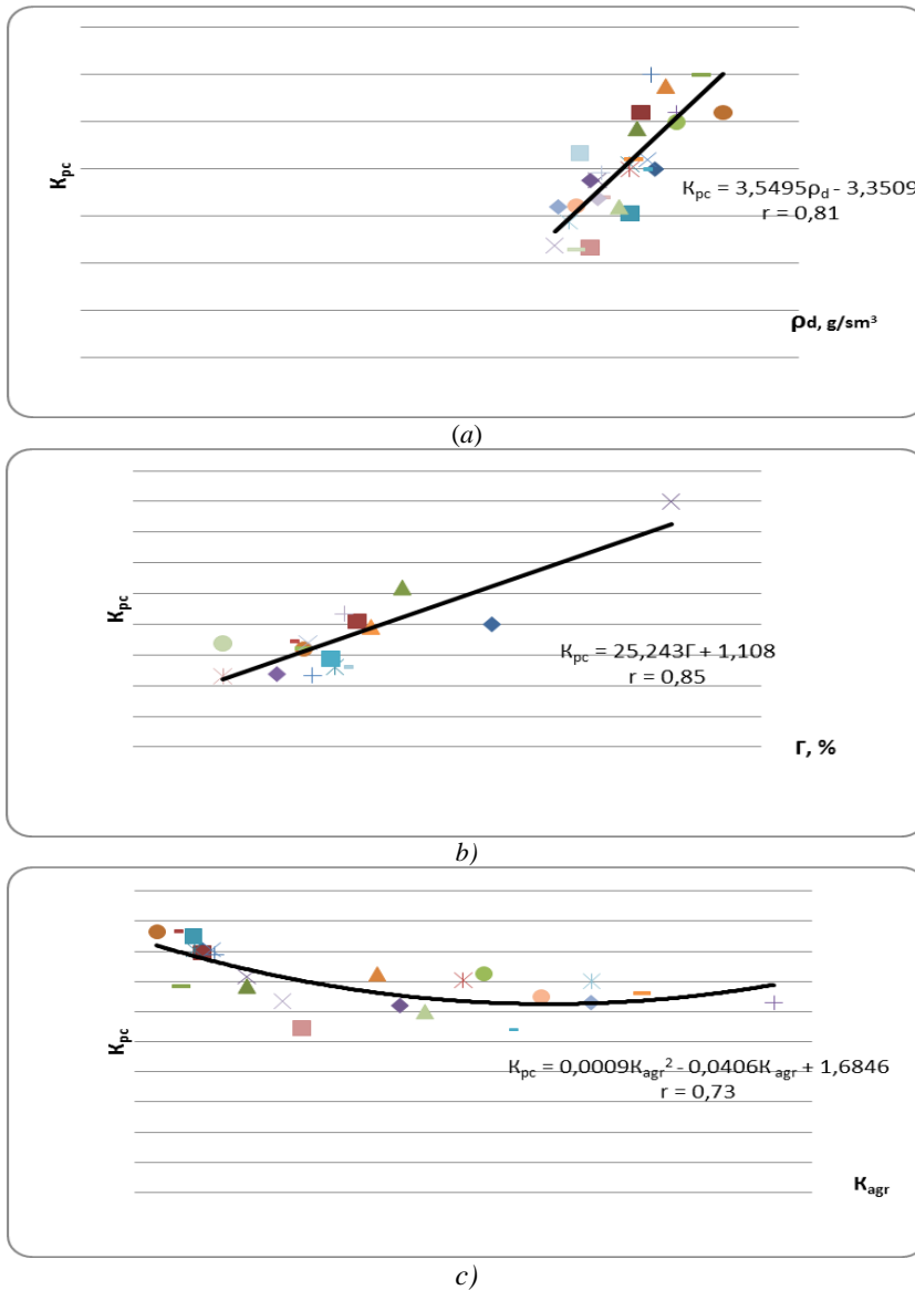
Fig. 1. Graphs of dependence of the coefficient of post-subsidence compaction the K_{pc} from the density of dry soil \rho_d (a), content of gypsum G (b), coefficient of aggregation of the disperse fraction K_{agr} (c).
