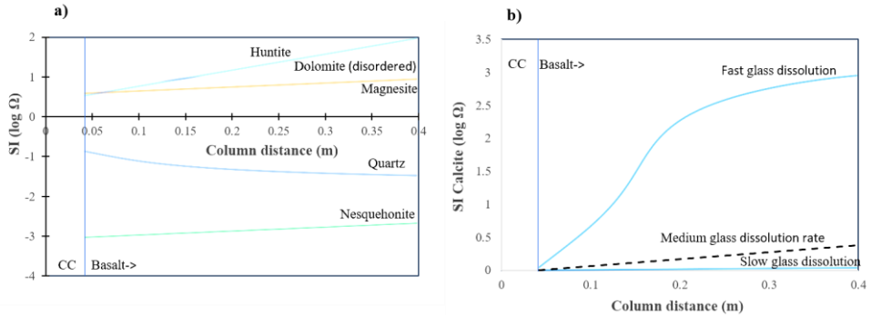
Fig. 3. PHREEQC v3 simulated saturation states of reacted solutions with respect to a) possible solid carbonates using the mid-range basalt dissolution rate ( k = 1.0 \times 10^{-9.0} mol/m 2 s); and b) calcite at three different basalt dissolution rates; fast ( k = 1.0 \times 10^{-8.0} mol/m 2 s), medium ( k = 1.0 \times 10^{-9.0} mol/m 2 s), and slow ( k = 1.0 \times 10^{-10.0} mol/m 2 s). The snapshots are taken at 1.0 pore volumes of flow.
