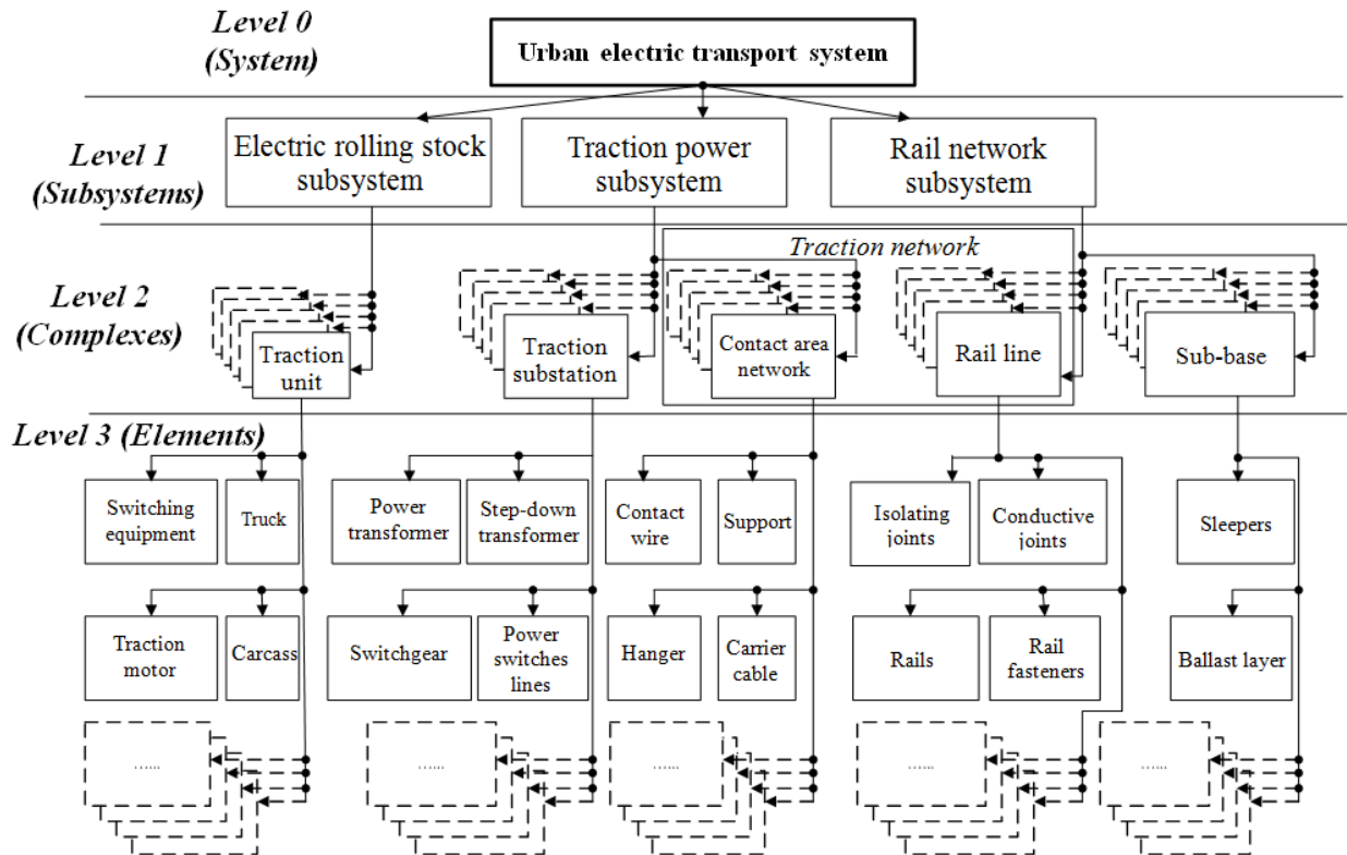
Fig. 2. Decomposition of the electric transport system of the urban agglomeration.
