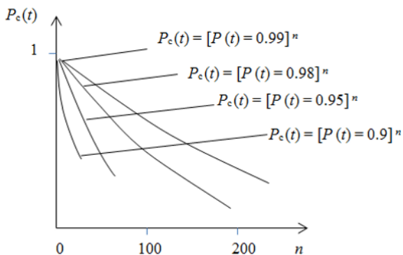
Fig. 5. Change in the reliability of the system depending on the reliability of elements and the number of elements n .
