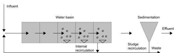
Fig. 1. Illustration of Sewon Bantul WWTP
