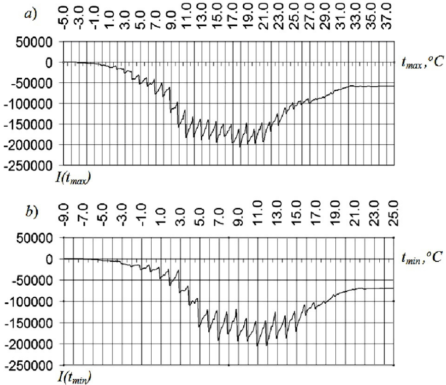
Fig. 2. Graphic of integral trends for maximum (a) and minimum (b) temperatures
