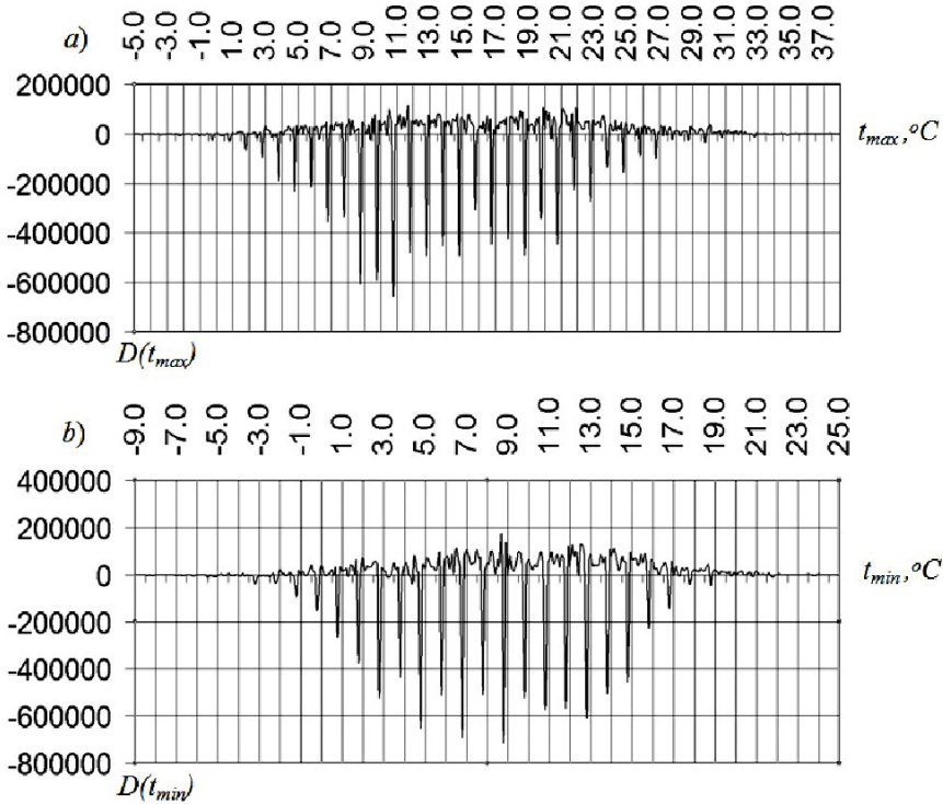
Fig. 3. Graphics of differential trend in the maximum (a) minimum and (b) temperatures in London during the period from 01.01.1973 on 31.08.2009.
