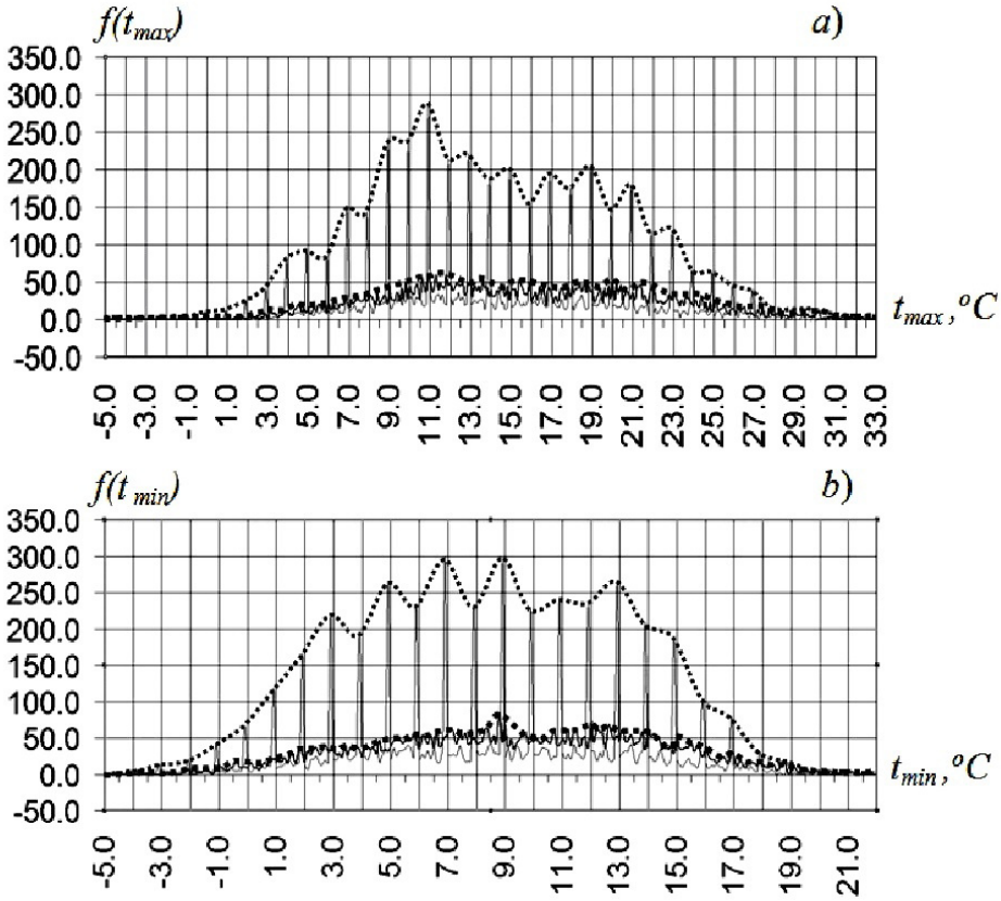
Fig. 1. Statistical distribution curves on a temperature scale the realizing events number of the maximum (a) and minimum (b) daily temperatures, f(t_{max}) and f(t_{min}) , in London: the thin lines show the curves corresponding to data in the period from 01.01.1973 on 01.01.1994 and the thin bold line - in the period from 31.08.1994 – 31.08.2009; bold lines represent the envelope curves of the corresponding statistical distribution
