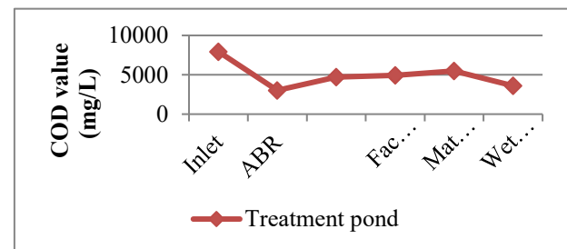
Fig.3. COD 5 value in Temesi leachate treatment plant
