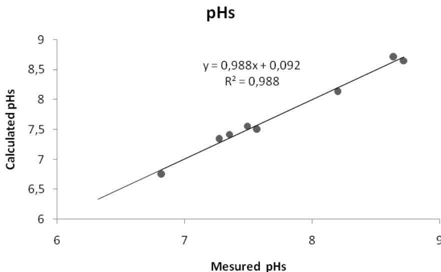
Fig. 4. Calculated values line according to the actual values of response pHs
