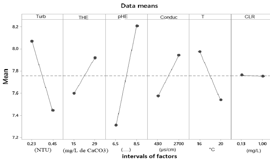
Fig.1. The effects of drinking water parameters on the response pH (pHs)
