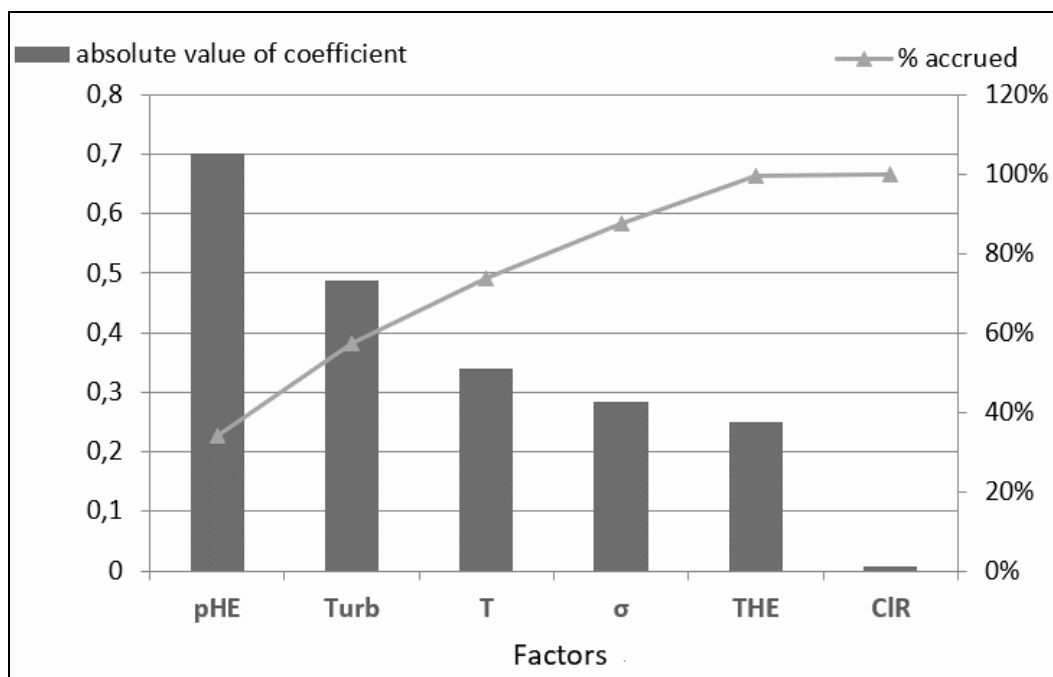
Fig. 2. Response pHs Pareto diagram
