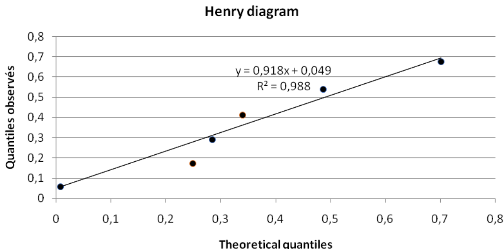
Fig. 3. Henry diagram of response pHs
