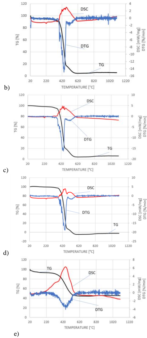
Fig. 3. DSC/TG/DTG curves of: a) PA6 9 (polyamide), b) PA6+1%M, c) PA6+3%M, d) PA6+5%M, e) M (coal sludge)
