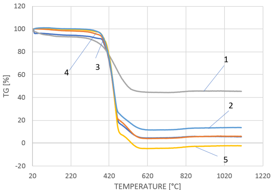
Fig. 6. TG curves of samples; 1 - M (coal sludge), 2- PA6 9 (polyamide), 3 - PA6+1%M, 4 - PA6+3%M, 5 - PA6+5%M
