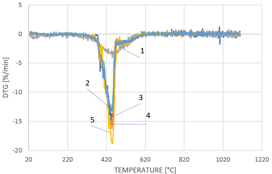
Fig. 5. DTG curves of samples; 1 - M (coal sludge), 2- PA6 9 (polyamide), 3 - PA6+1%M, 4 - PA6+3%M, 5 - PA6+5%M
