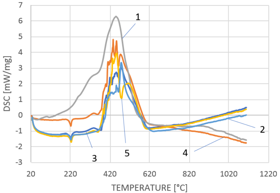
Fig. 4. DSC curves of samples; 1 - M (coal sludge), 2- PA6 9 (polyamide), 3 - PA6+1%M, 4 - PA6+3%M, 5 - PA6+5%M
