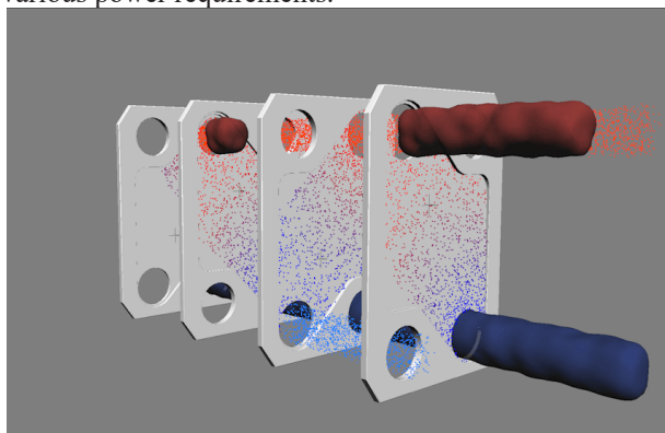
Figure 1. Working principle of temperature difference semiconductor
