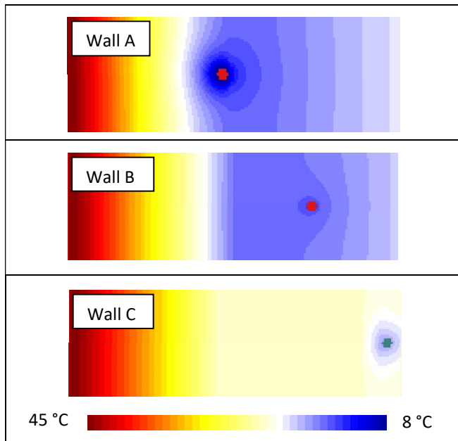
Fig. 4. Temperature distribution within wall fragments of the three wall cooling systems.
