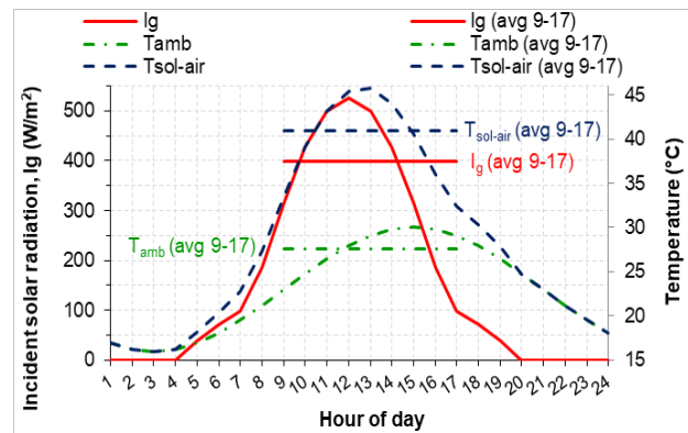
Fig. 2. The course of sol-air temperature, ambient temperature and intensity of solar radiation during the design day.
