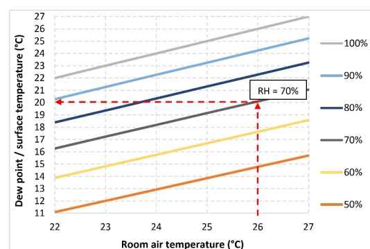
Fig. 3. Dew point temperature for various combinations of room air temperature and relative air humidity.
