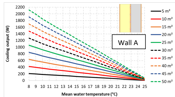
Fig. 5. Effect of water temperature on the cooling output at various cooling surface areas (Wall A).
