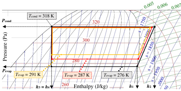
Fig. 11. Effect of evaporation temperature on enthalpy difference h_2-h_1 for R410A (log(p)-h diagram).
