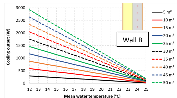
Fig. 6. Effect of water temperature on the cooling output at various cooling surface areas (Wall B).
