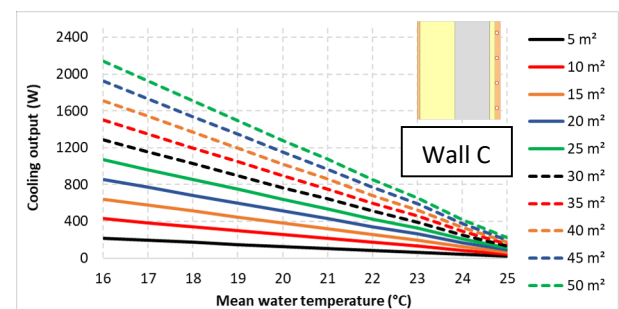
Fig. 7. Effect of water temperature on the cooling output at various cooling surface areas (Wall C).
