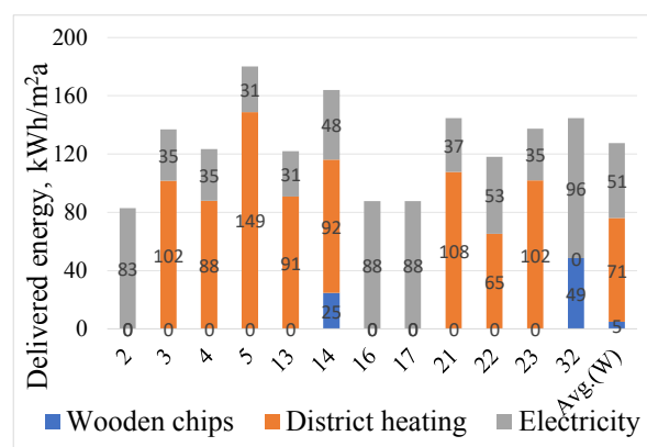
Fig. 8. Delivered energy of district buildings.
