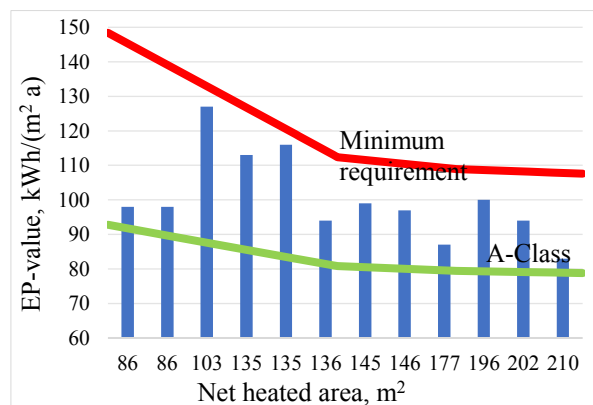
Fig. 3. EP-value in 12 detached houses.
