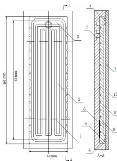
1 Evaporating section, 2 Middle section, 3 Condensing section, 4 Seal groove, 5 Resistor, 6 Adiabetic base, 7 Cooling water channels, 8 Aluminum flat plate, 9 Slit, 10 Flow channel, 11 Plexiglas cover
