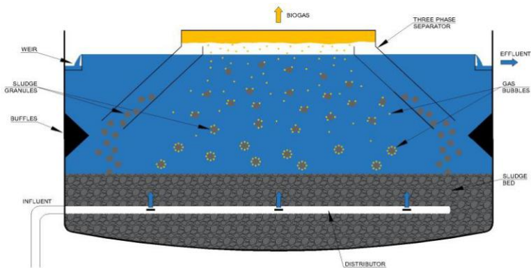
Fig. 1. UASB reactor
