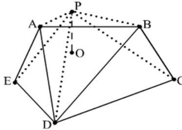
Fig. 10. The example of removing the vertex P and 5 triangles incident to it followed by filling the gap with three triangles.
