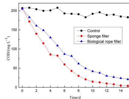
Fig. 2. The removal effect of bionic plants on COD.
