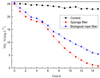
Fig. 3. The removal effect of bionic plants on \text{NH}_4^+\text{-N}
