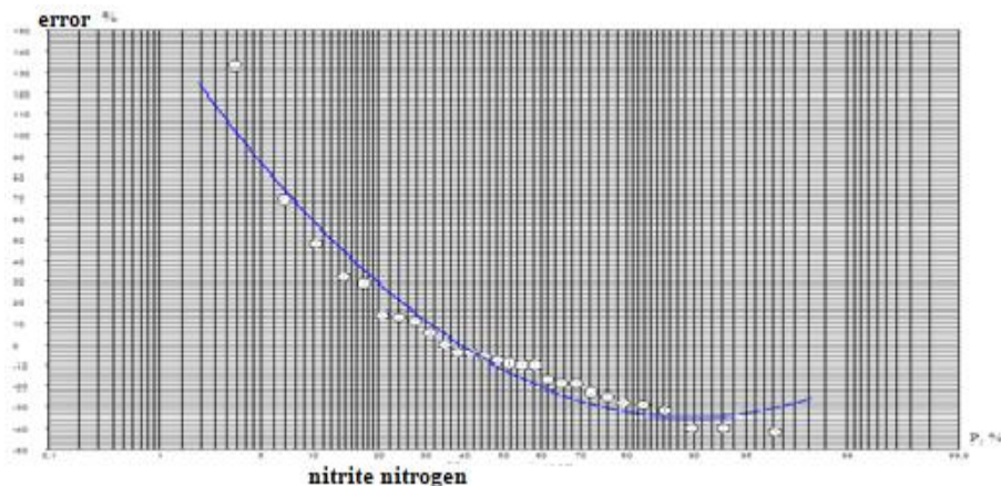
Fig. 5. Empirical curve of provision of generalized series of errors \delta_i (%) for calculating the average annual concentration of nitrite nitrogen, taking into account water content.
