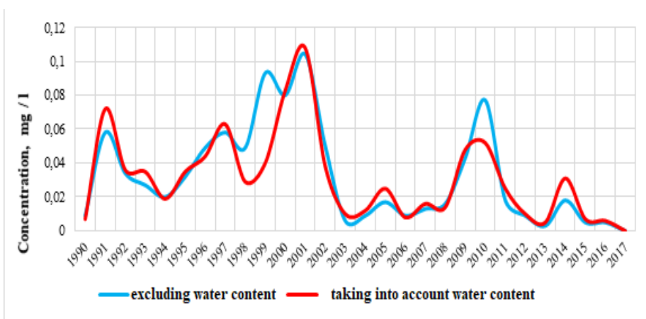
Fig. 3. Average annual concentrations of nitrite nitrogen with and without water content at station 101 point-1217401 of the Pskem river, Mullala village, section 01
