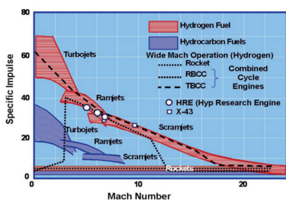
Figure 1. Variation of specific impulse with flight Ma for each engine type (Image from the web)
