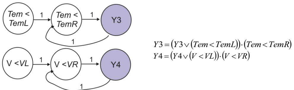
Fig. 4. Graph-diagram diagram of the heater and fan control.
