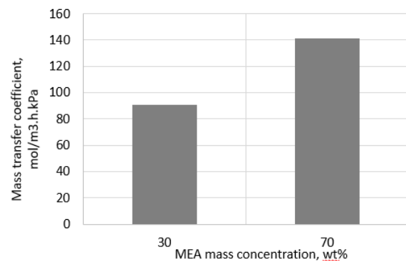
Figure 1 Effect of MEA concentration on mass transfer coefficient
