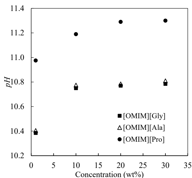
Fig. 1: pH measurement of AAILs solutions with respect to concentration.
