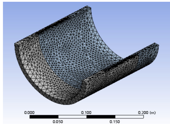
Figure 2. Meshing result diagram
