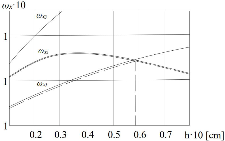
Fig.2. Plot of damping coefficients versus natural modes.
