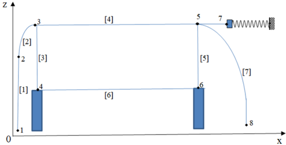
Fig.1 Calculation scheme of the shell structure
